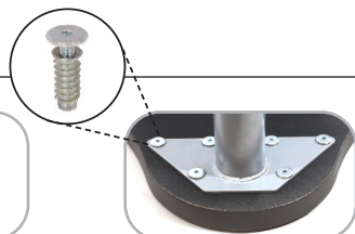
Legs positioned at widest point of table for stability and attached via threaded metal inserts and bolts
